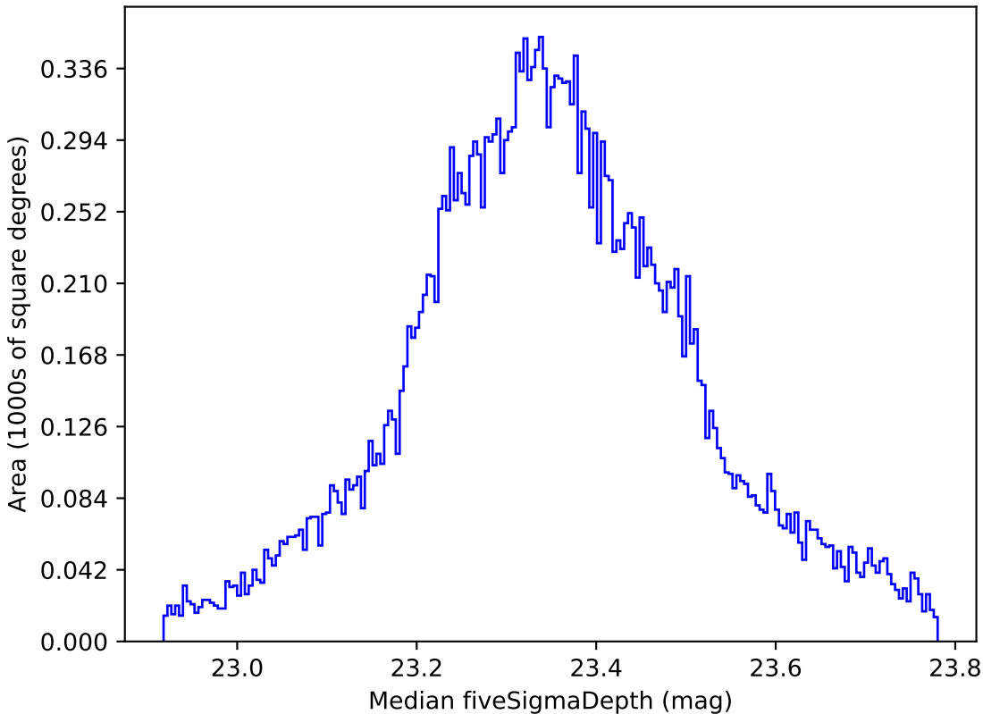
smc_lmc_v3.3_10yrs All sky all bands: Median fiveSigmaDepth
