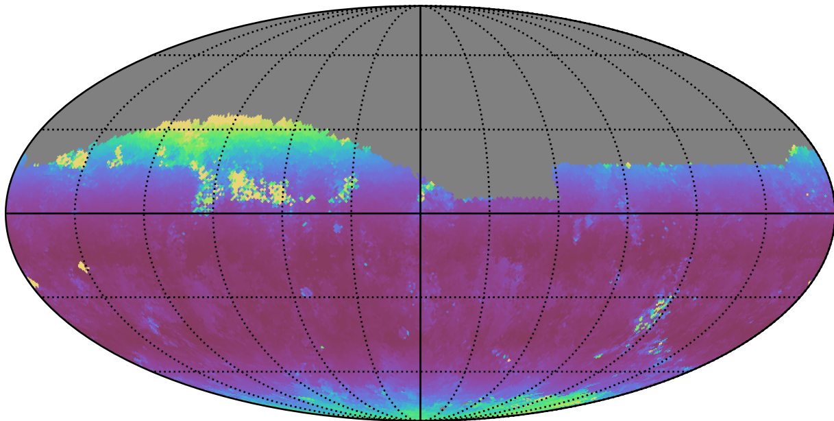
smc_lmc_v3.3_10yrs Yr 1 z band: Median airmass
