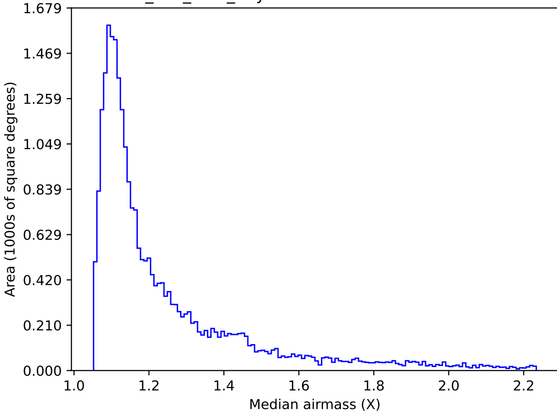
smc_lmc_v3.3_10yrs Yr 1 z band: Median airmass
