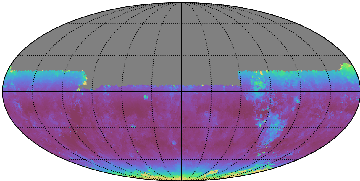
smc_lmc_v3.3_10yrs Yr 1 y band: Median airmass
