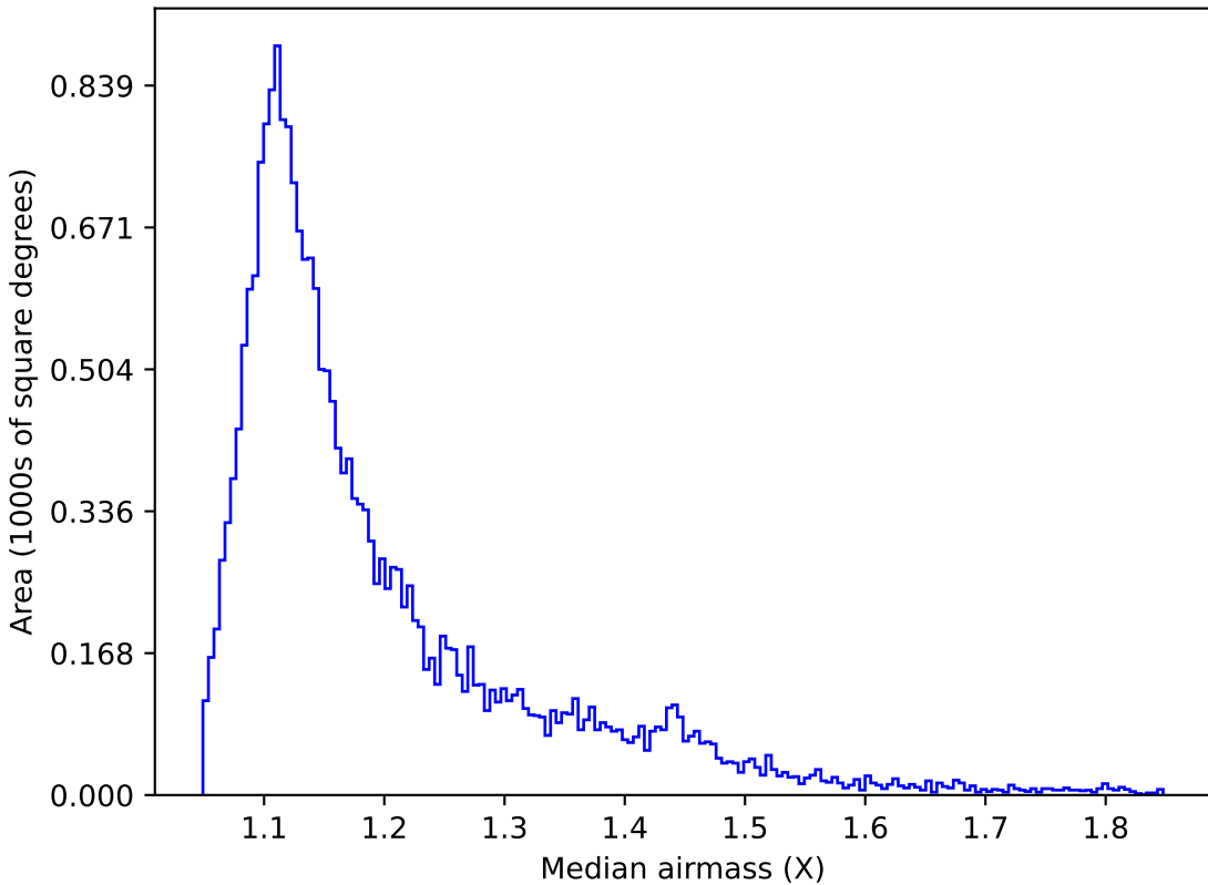
smc_lmc_v3.3_10yrs Yr 1 y band: Median airmass
