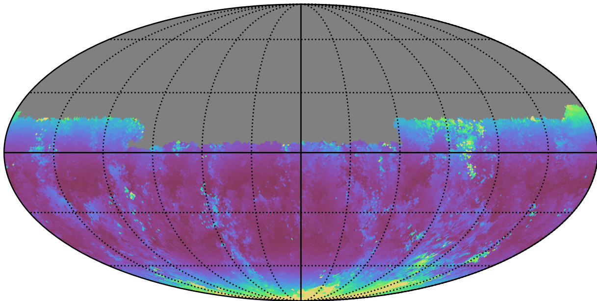
smc_lmc_v3.3_10yrs Yr 1 u band: Median airmass
