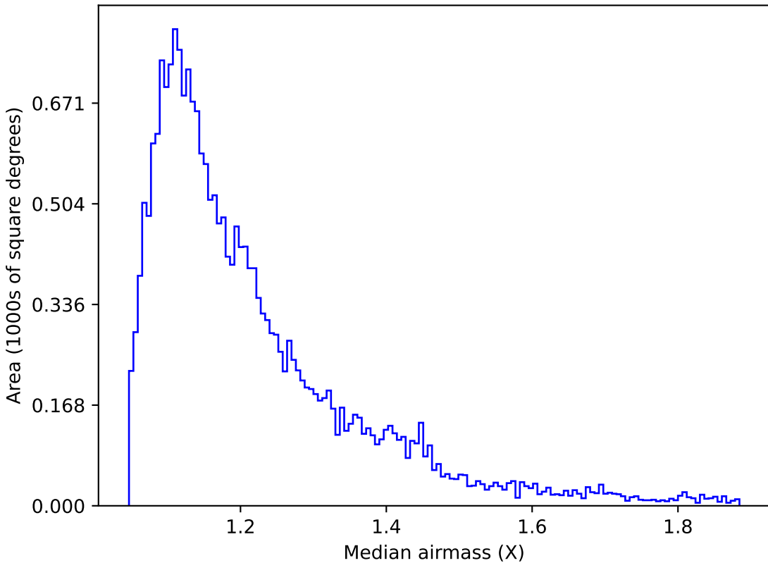
smc_lmc_v3.3_10yrs Yr 1 u band: Median airmass
