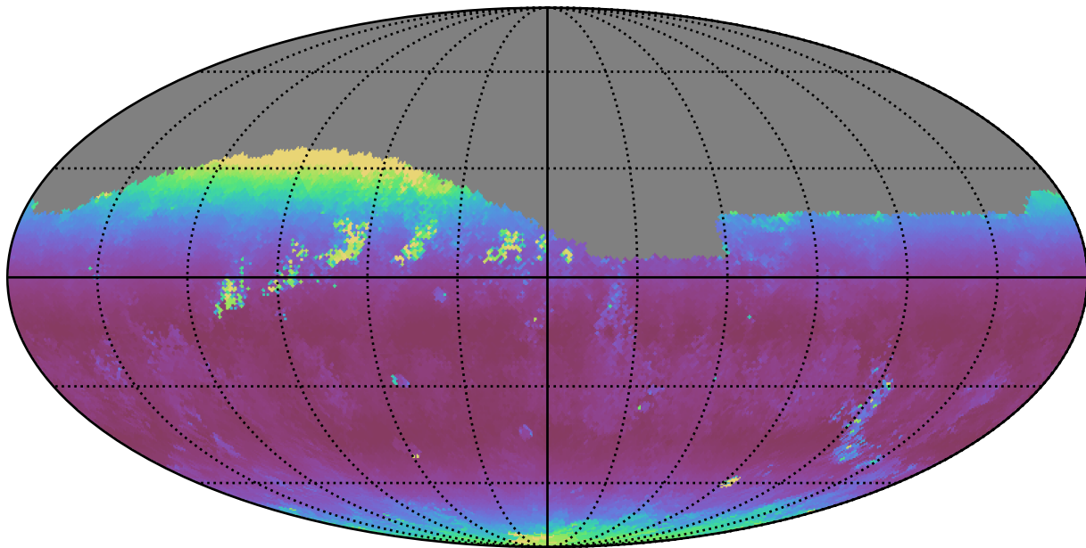
smc_lmc_v3.3_10yrs Yr 1 r band: Median airmass
