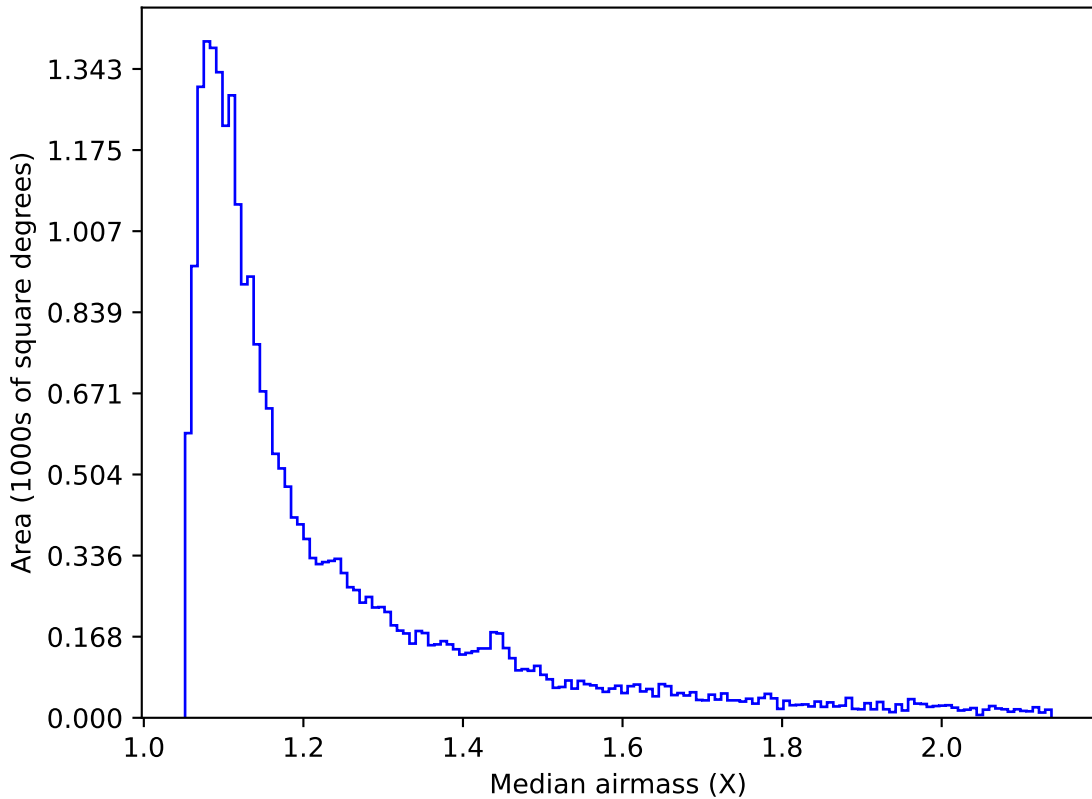
smc_Imc_v3.3_10yrs Yr 1 r band: Median airmass
