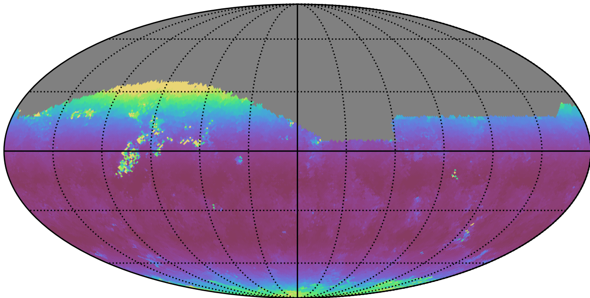
smc_lmc_v3.3_10yrs Yr 1 i band: Median airmass
