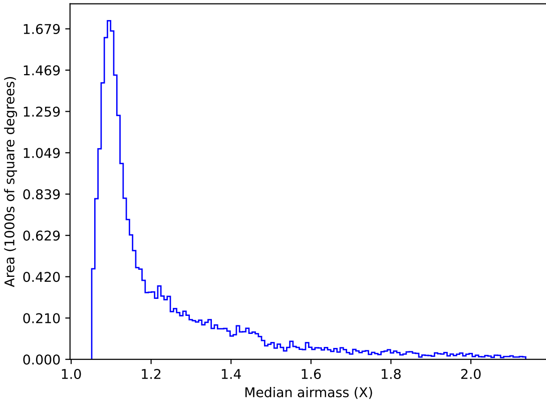
smc_lmc_v3.3_10yrs Yr 1 i band: Median airmass
