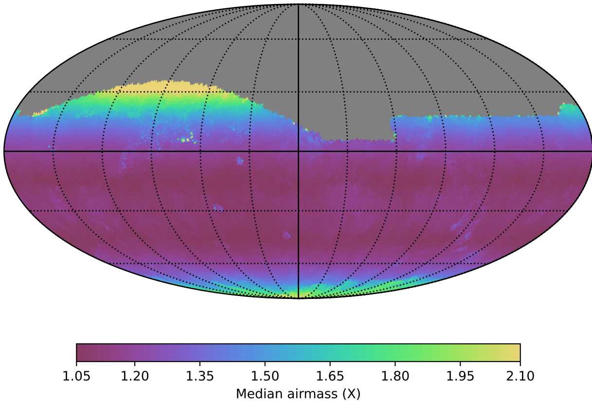
smc_lmc_v3.3_10yrs Yr 1 all bands: Median airmass
