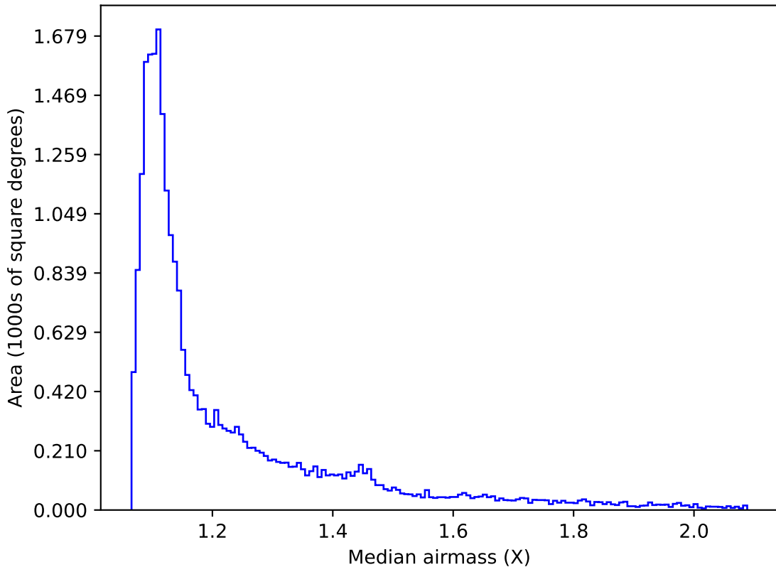
smc_lmc_v3.3_10yrs Yr 1 all bands: Median airmass
