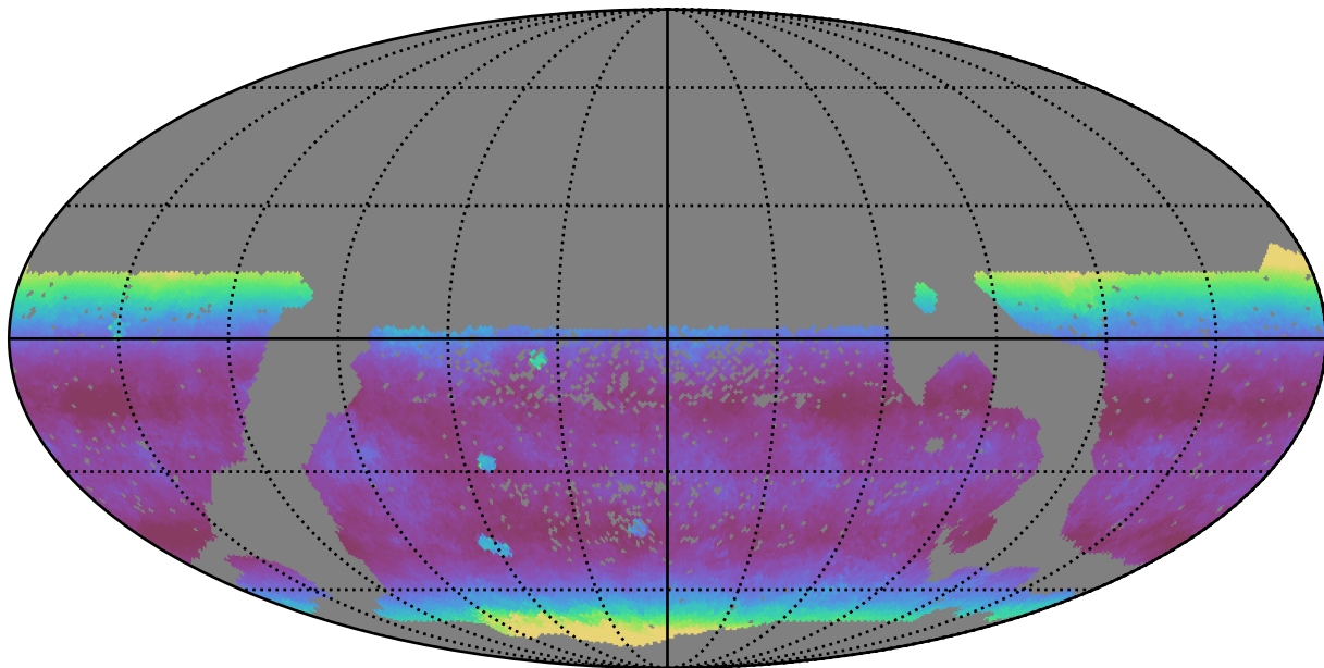
smc_lmc_v3.3_10yrs WFD z band: Median airmass
