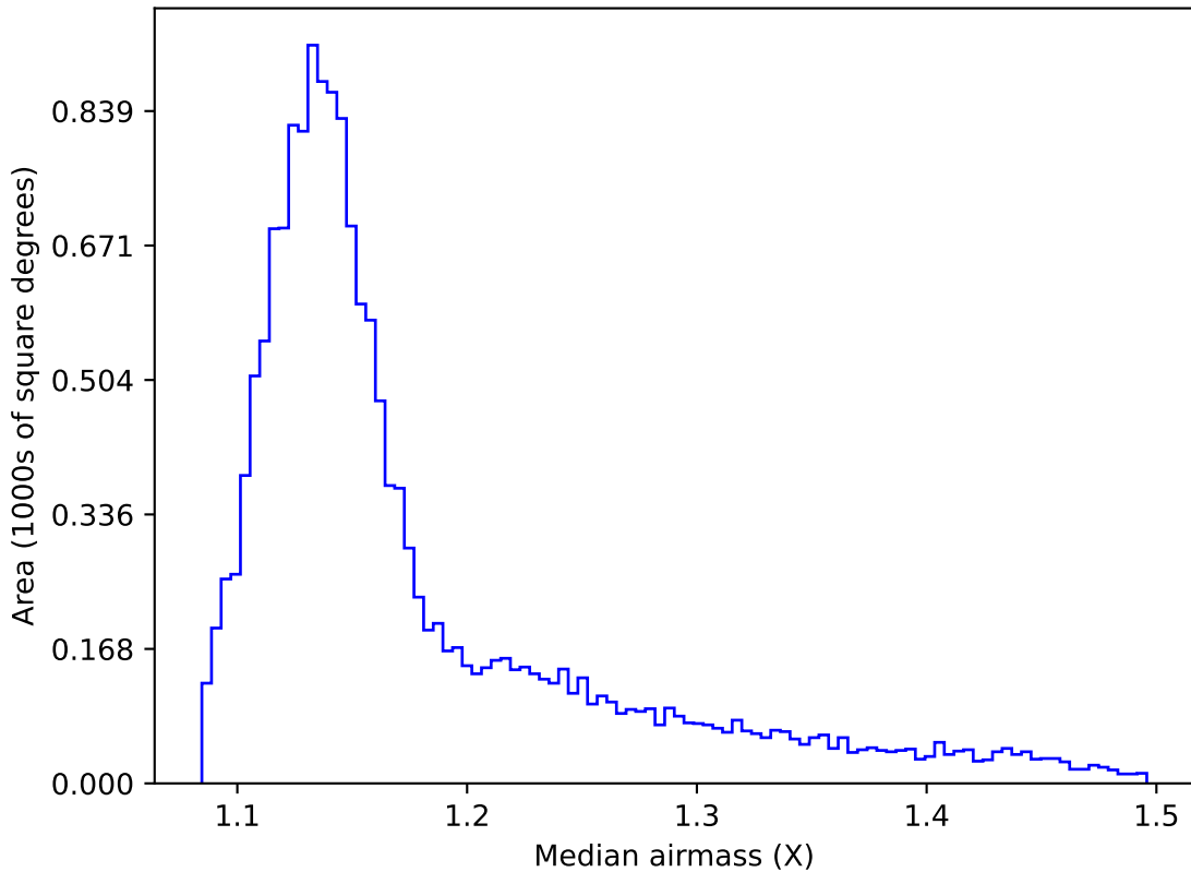
smc_lmc_v3.3_10yrs WFD z band: Median airmass
