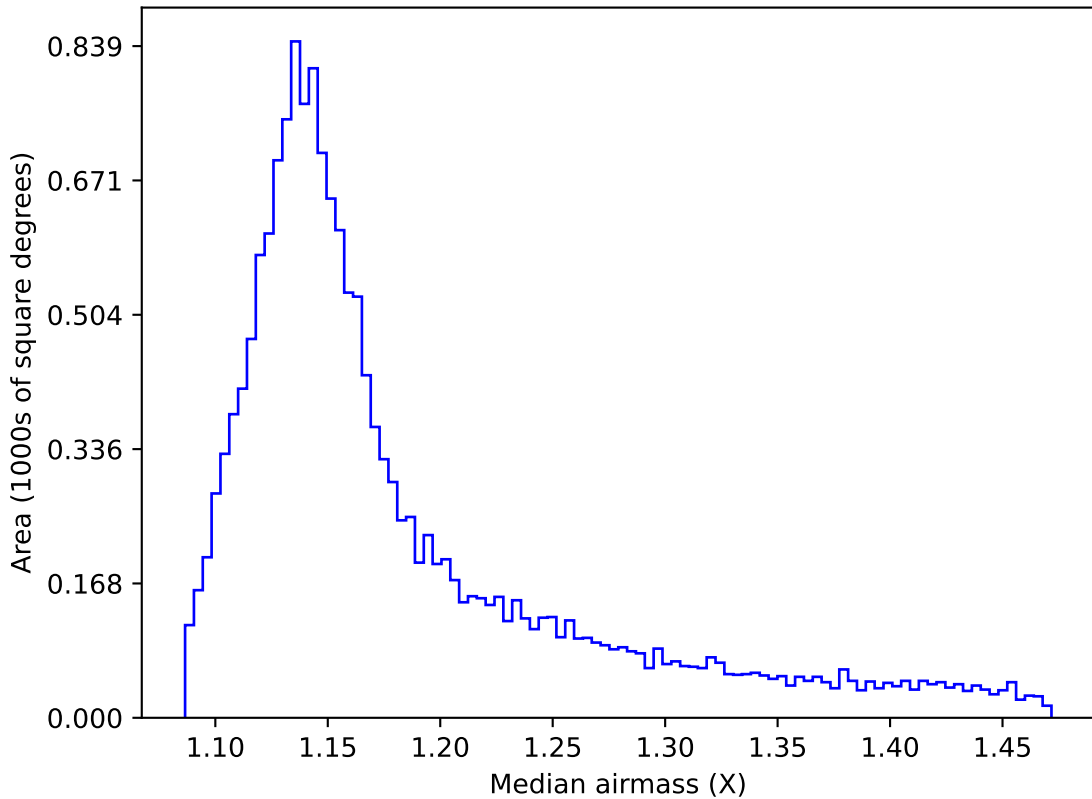
smc_lmc_v3.3_10yrs WFD y band: Median airmass
