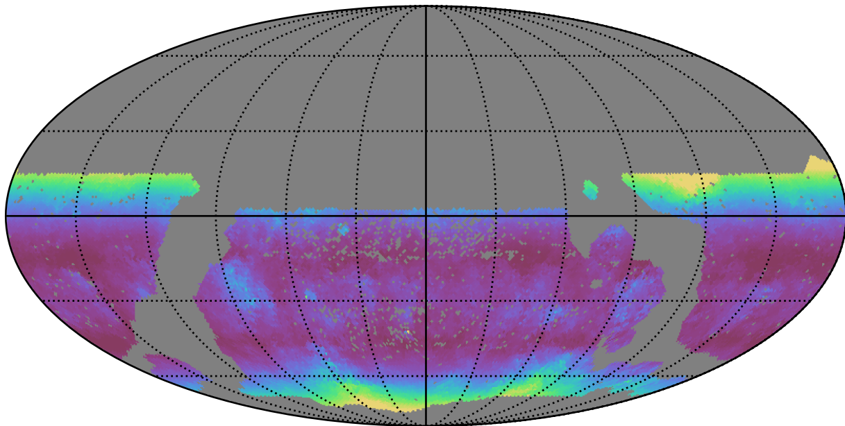
smc_lmc_v3.3_10yrs WFD u band: Median airmass
