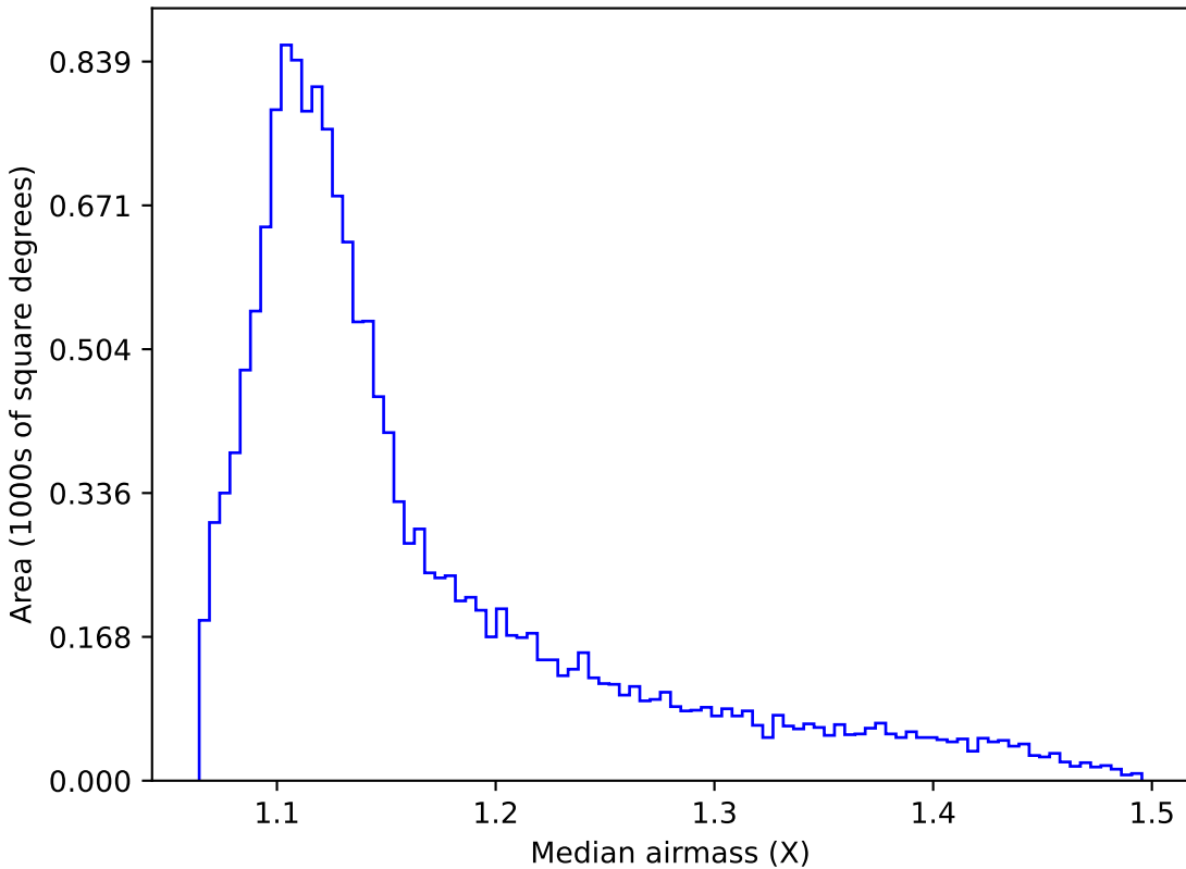
smc_lmc_v3.3_10yrs WFD u band: Median airmass
