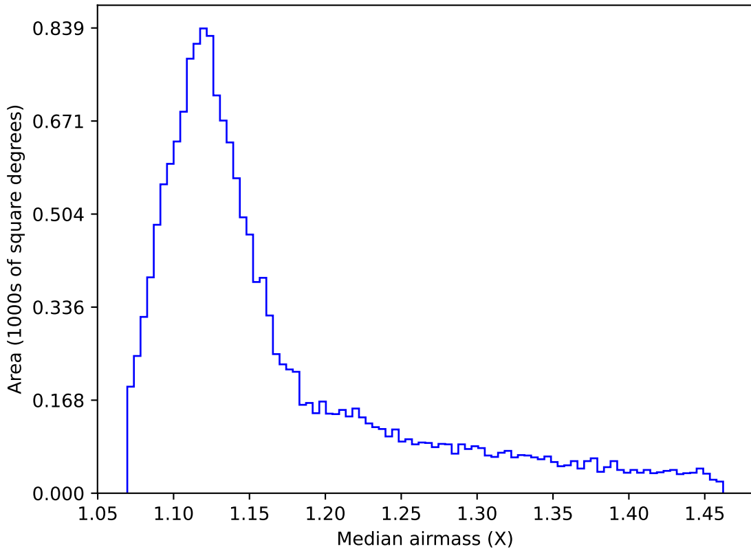
smc_lmc_v3.3_10yrs WFD r band: Median airmass
