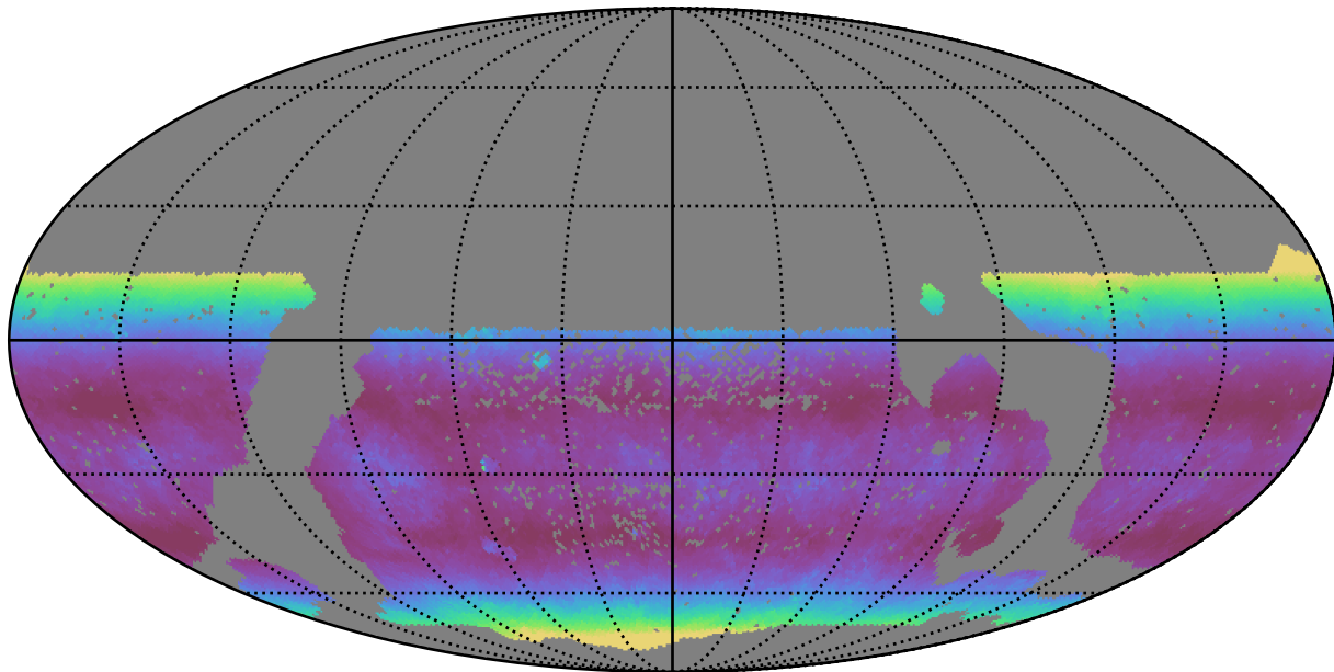
smc_lmc_v3.3_10yrs WFD i band: Median airmass
