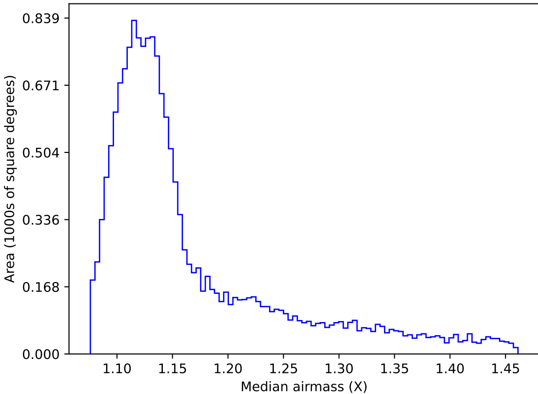
smc_lmc_v3.3_10yrs WFD i band: Median airmass
