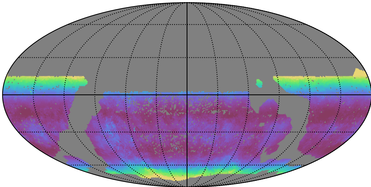
smc_lmc_v3.3_10yrs WFD g band: Median airmass
