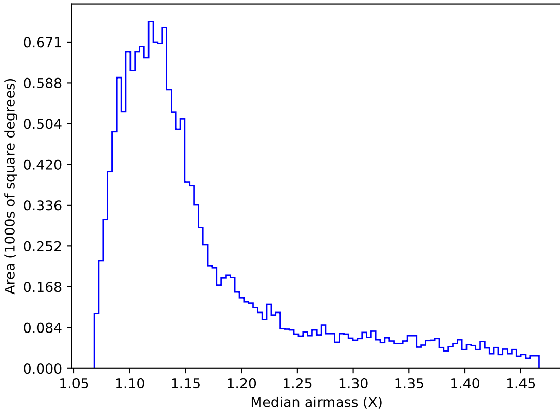
smc_lmc_v3.3_10yrs WFD g band: Median airmass
