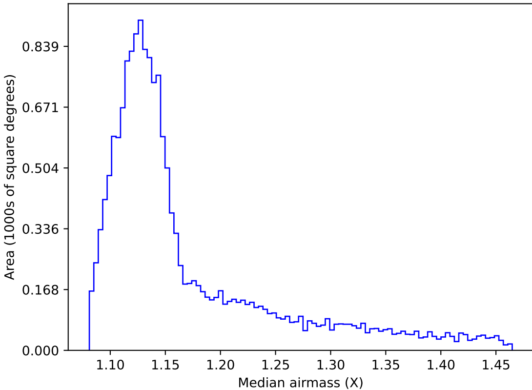
smc_lmc_v3.3_10yrs WFD all bands: Median airmass
