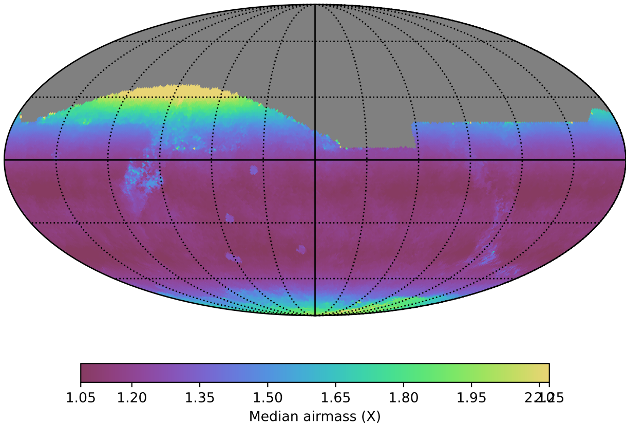
smc_lmc_v3.3_10yrs All sky z band: Median airmass
