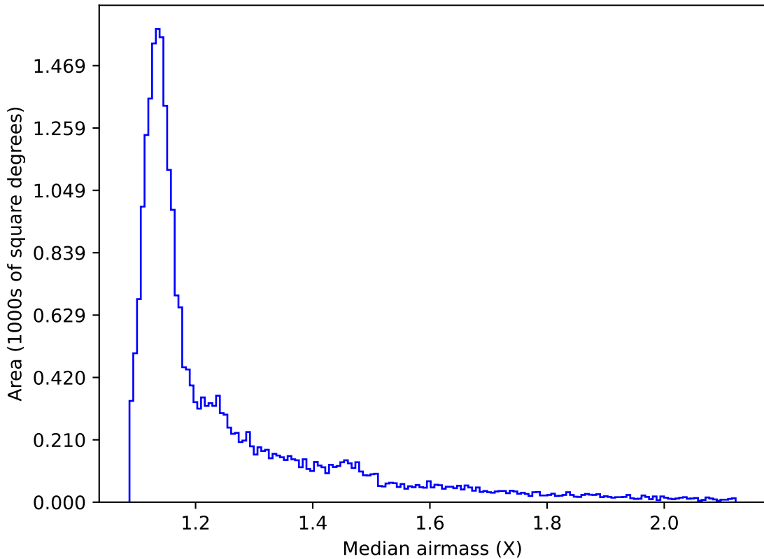
smc_lmc_v3.3_10yrs All sky z band: Median airmass
