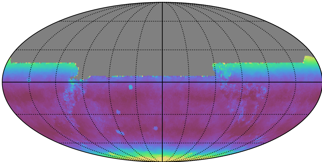
smc_lmc_v3.3_10yrs All sky y band: Median airmass
