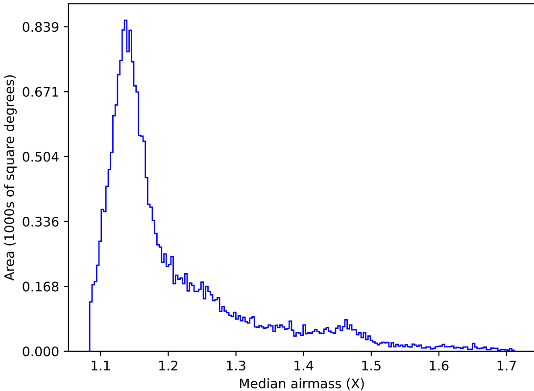
smc_lmc_v3.3_10yrs All sky y band: Median airmass
