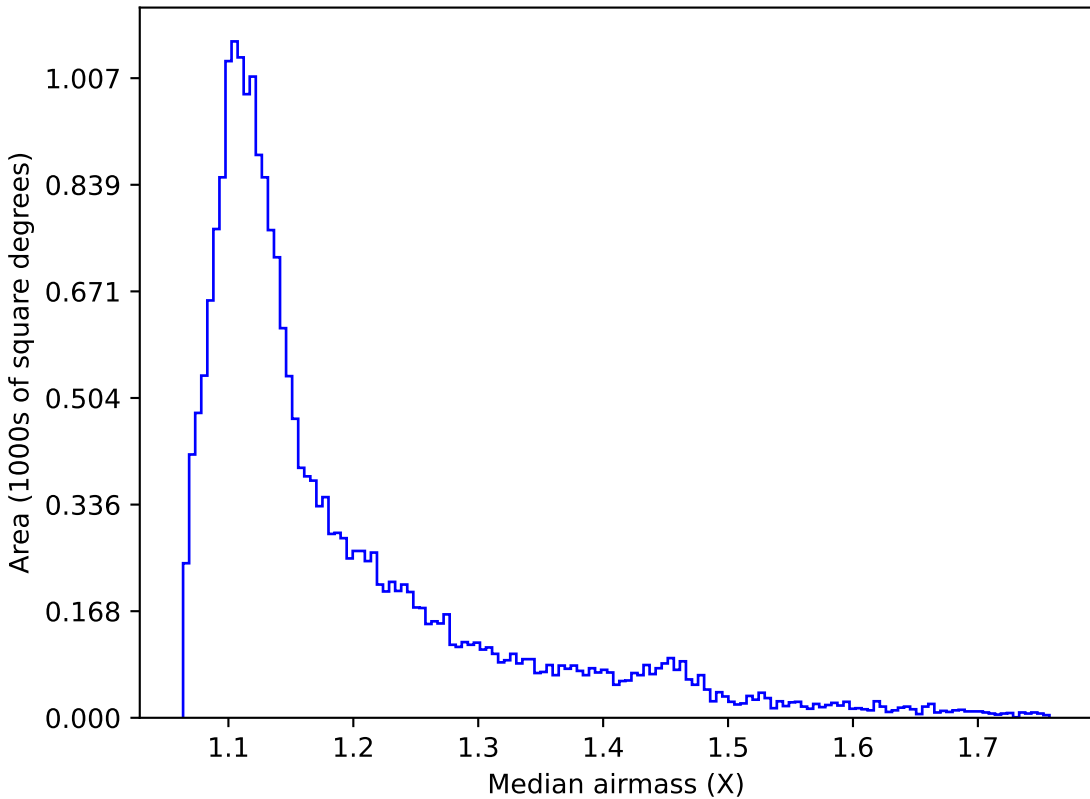
smc_lmc_v3.3_10yrs All sky u band: Median airmass
