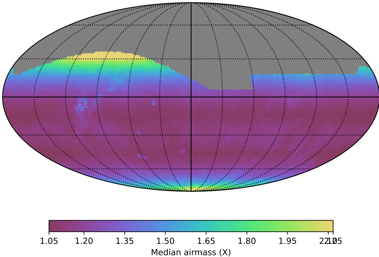
smc_lmc_v3.3_10yrs All sky r band: Median airmass
