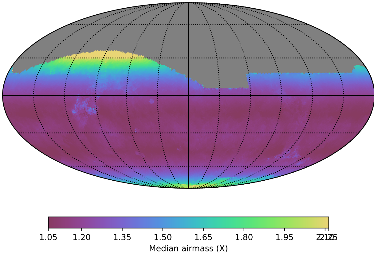
smc_lmc_v3.3_10yrs All sky i band: Median airmass
