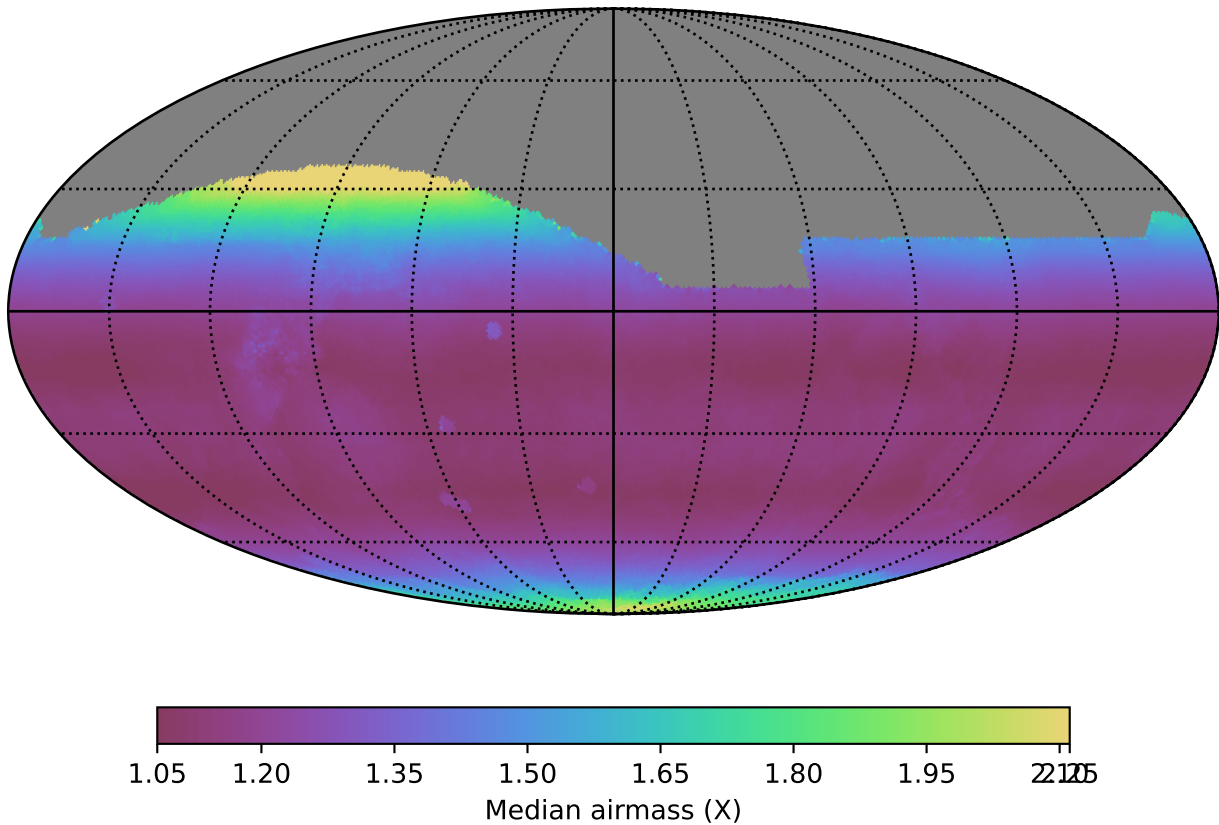
smc_lmc_v3.3_10yrs All sky all bands: Median airmass
