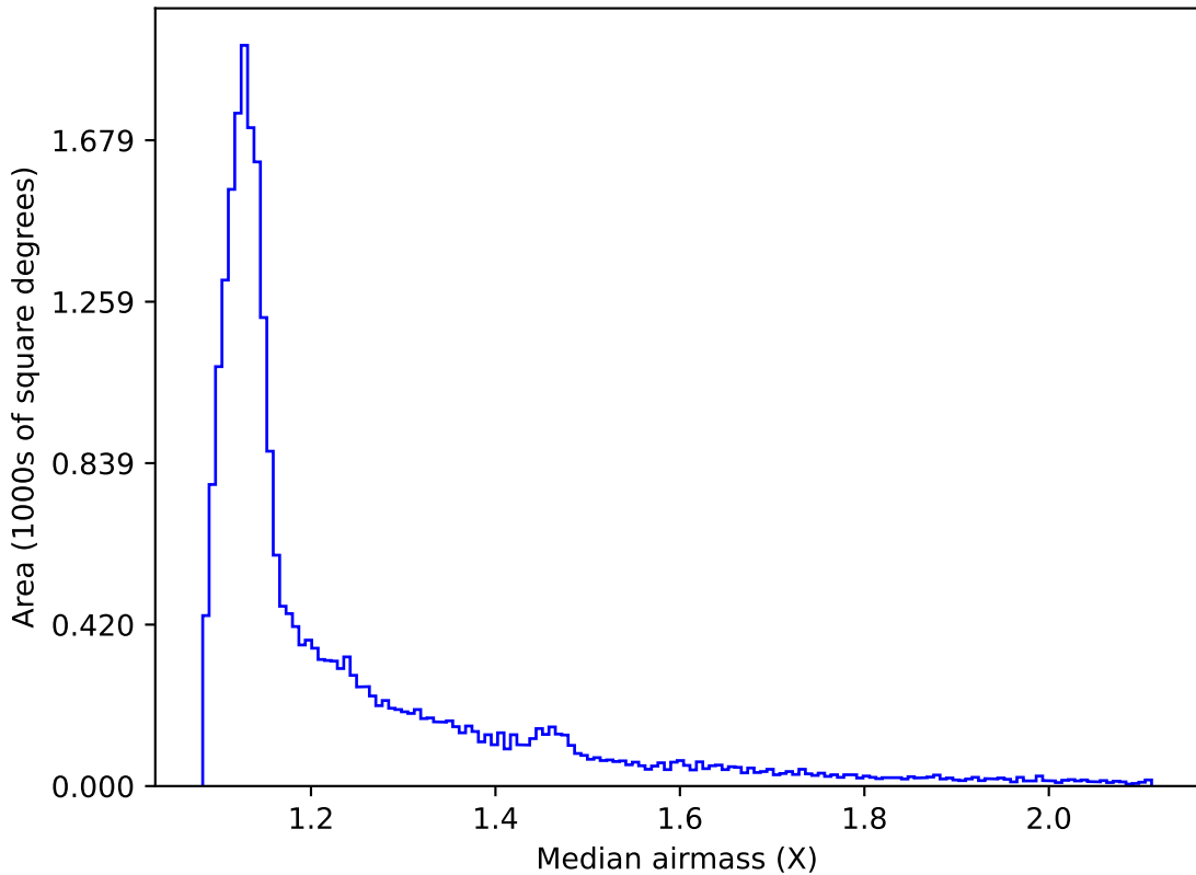
smc_lmc_v3.3_10yrs All sky all bands: Median airmass
