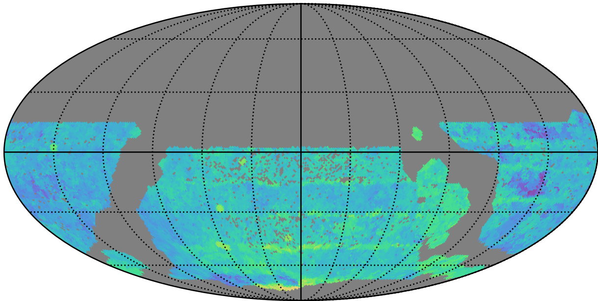
smc_lmc_v3.3_10yrs WFD z band: Median Season Length
