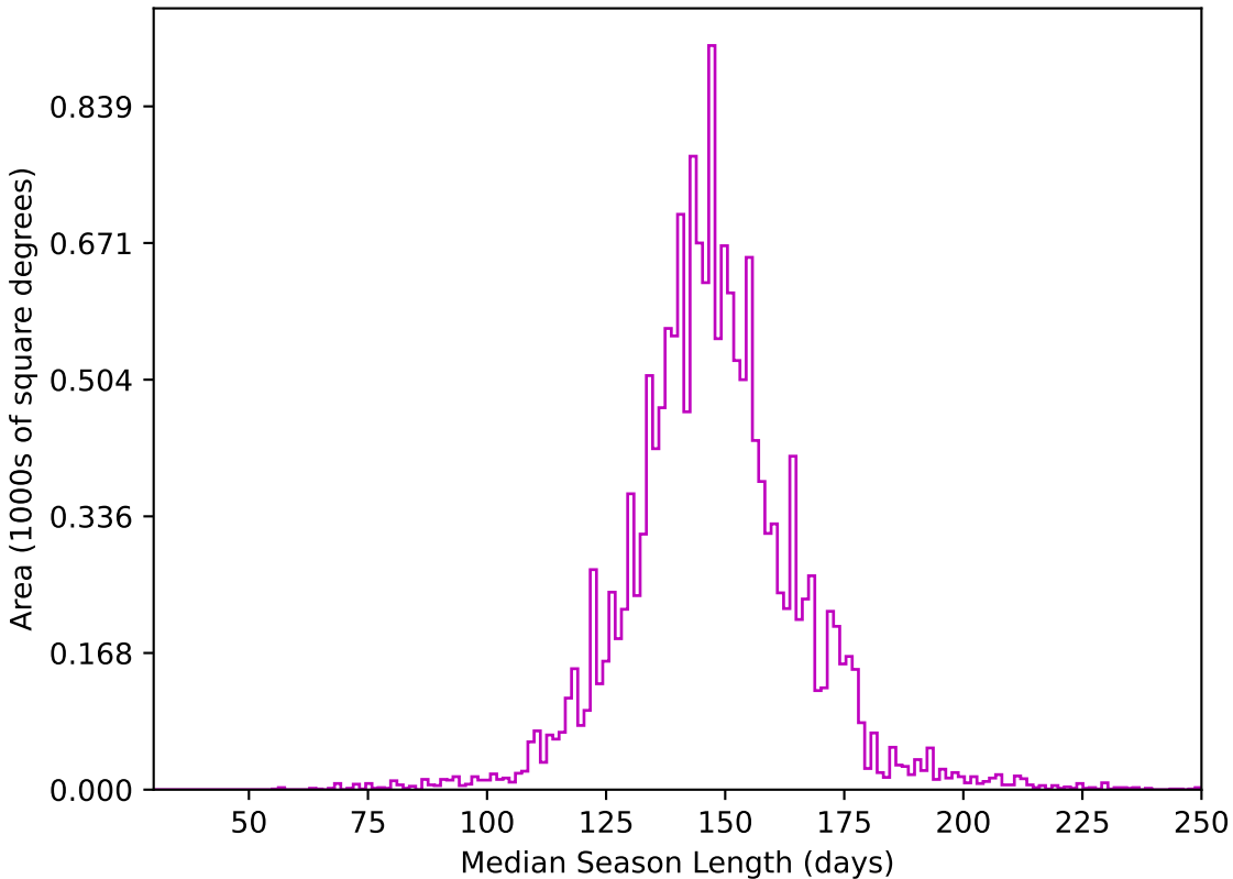
smc_lmc_v3.3_10yrs WFD z band: Median Season Length
