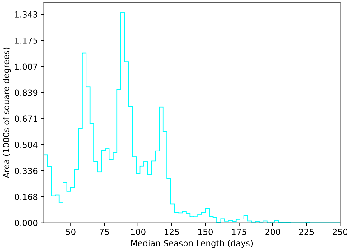
smc_lmc_v3.3_10yrs WFD u band: Median Season Length
