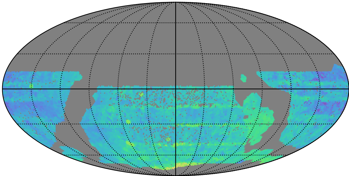
smc_lmc_v3.3_10yrs WFD r band: Median Season Length
