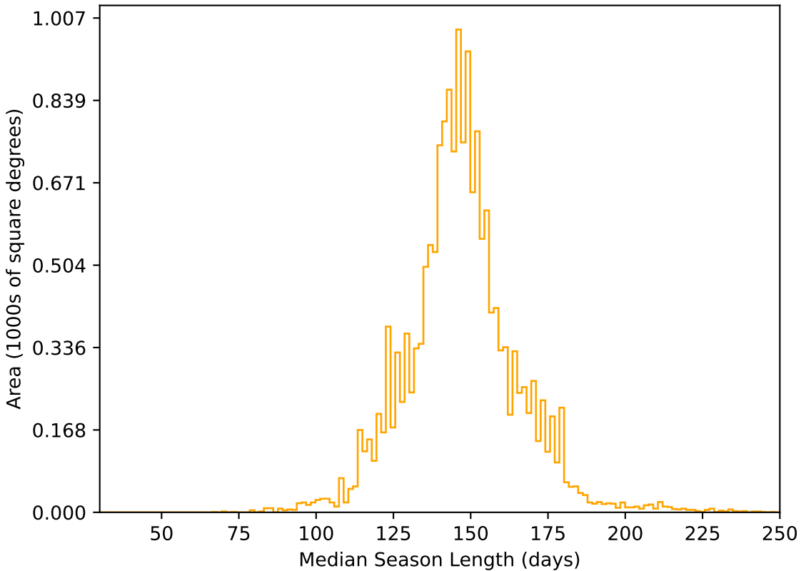
smc_lmc_v3.3_10yrs WFD r band: Median Season Length
