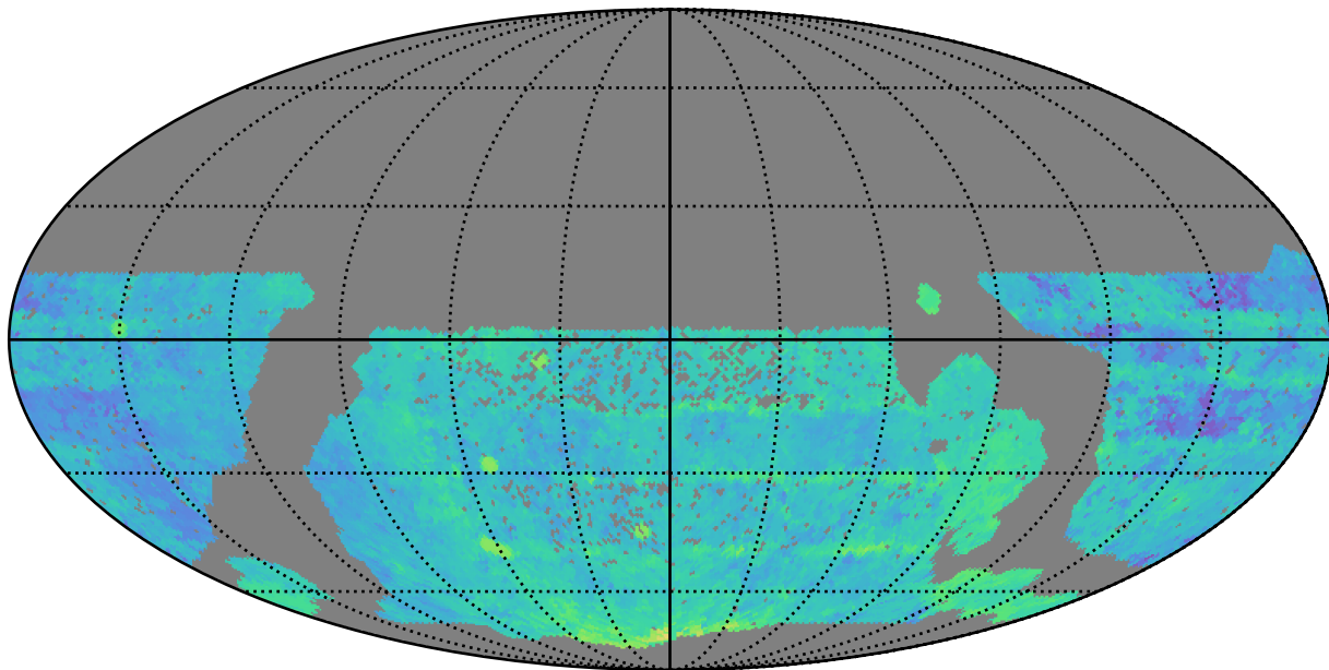
smc_lmc_v3.3_10yrs WFD i band: Median Season Length
