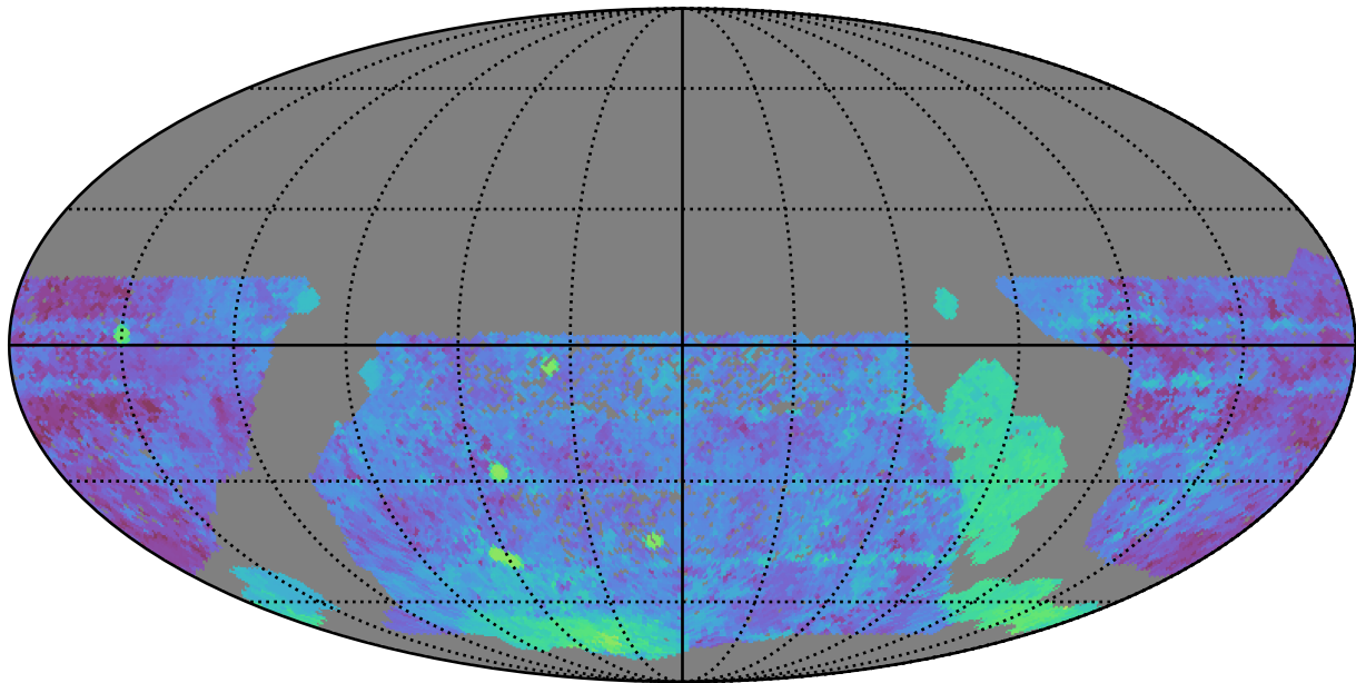
smc_lmc_v3.3_10yrs WFD g band: Median Season Length
