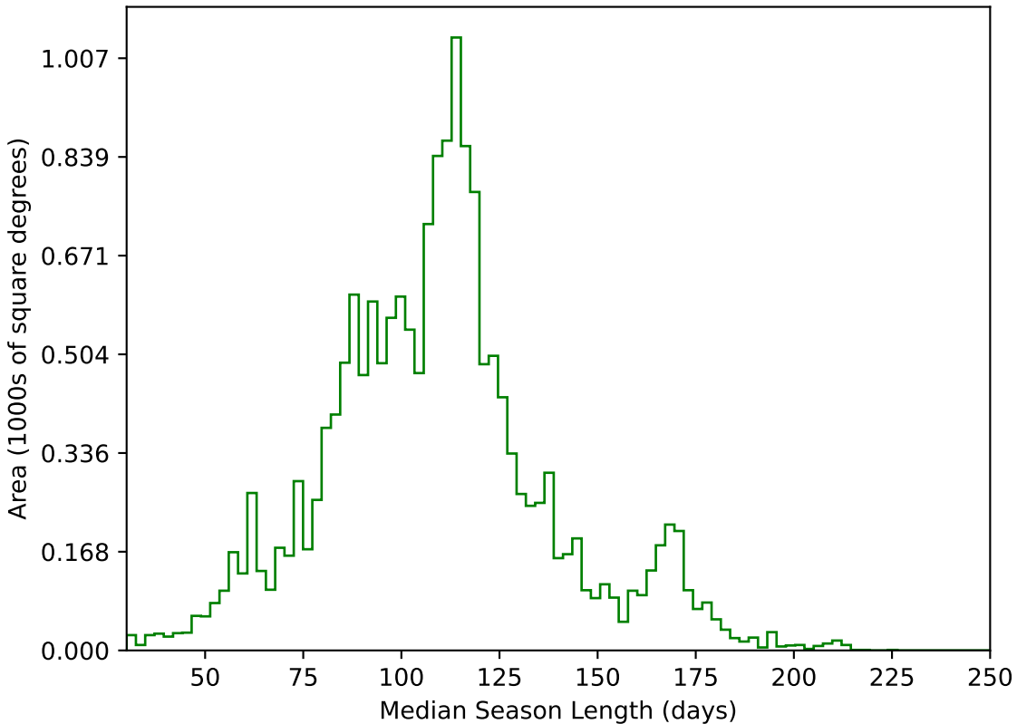
smc_lmc_v3.3_10yrs WFD g band: Median Season Length
