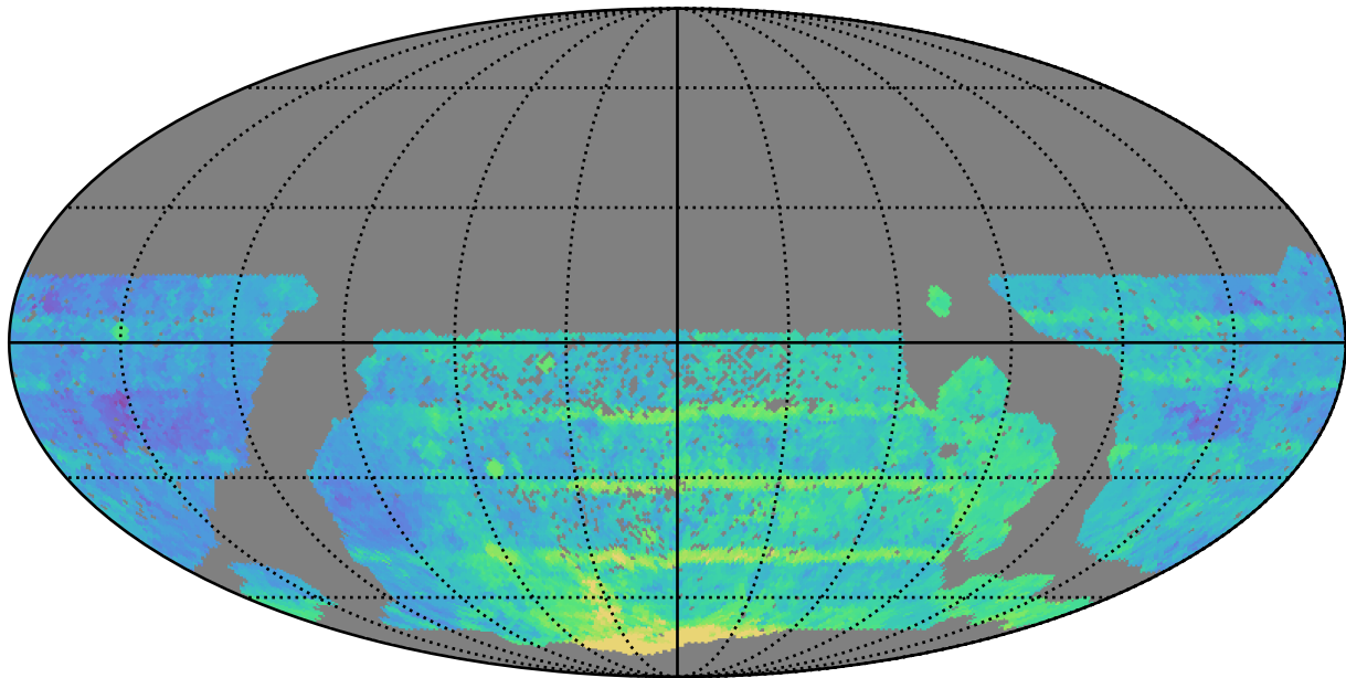
smc_lmc_v3.3_10yrs WFD all bands: Median Season Length
