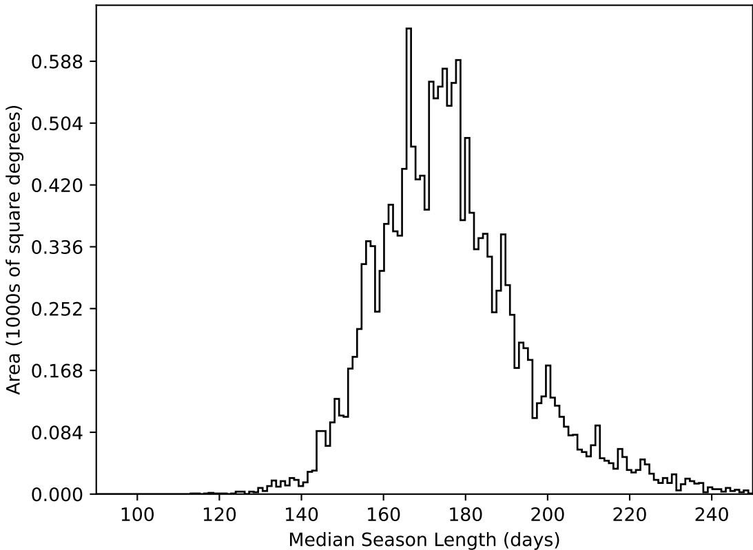
smc_lmc_v3.3_10yrs WFD all bands: Median Season Length
