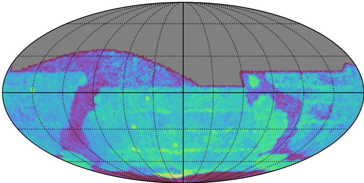
smc_lmc_v3.3_10yrs All sky z band: Median Season Length
