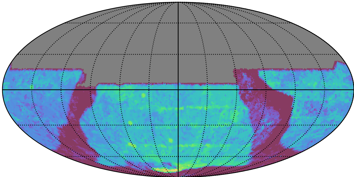
smc_lmc_v3.3_10yrs All sky y band: Median Season Length
