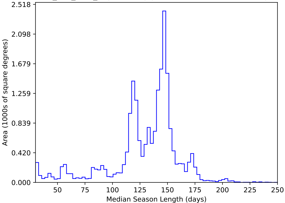
smc_lmc_v3.3_10yrs All sky y band: Median Season Length
