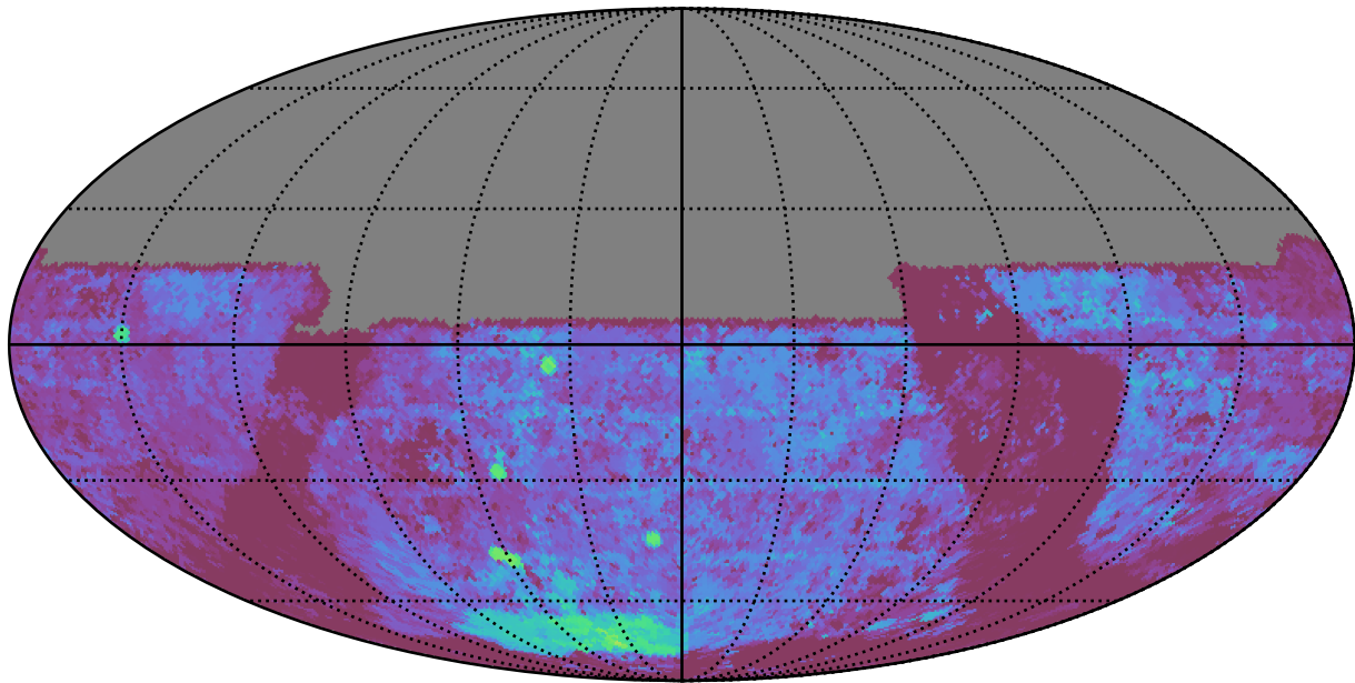
smc_lmc_v3.3_10yrs All sky u band: Median Season Length
