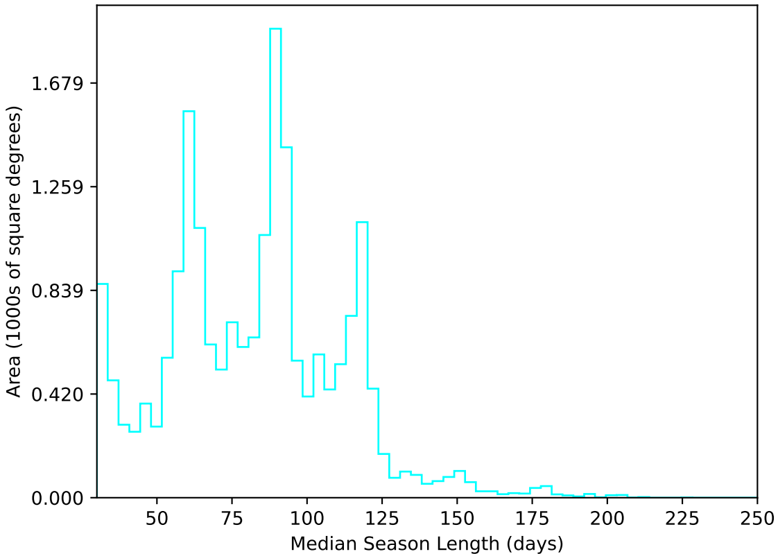
smc_lmc_v3.3_10yrs All sky u band: Median Season Length
