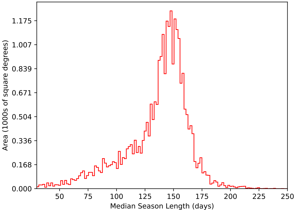
smc_lmc_v3.3_10yrs All sky i band: Median Season Length
