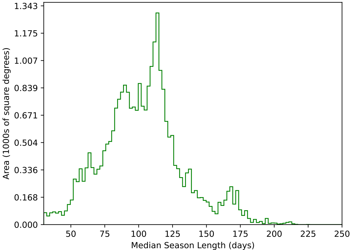
smc_lmc_v3.3_10yrs All sky g band: Median Season Length
